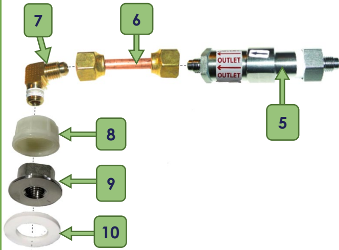
INLET ASSEMBLY FOR VALVE PN 111775 (Includes PNs 6-9 from table below)
