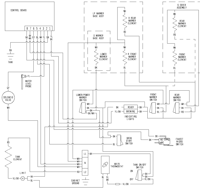
240V WARMER
