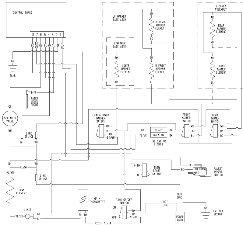
240V WARMER
