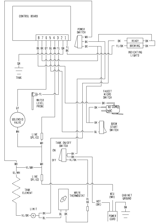
120V DISP.
