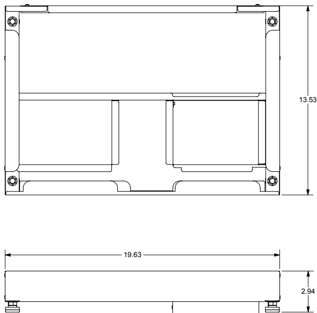
Dimensions of riser
