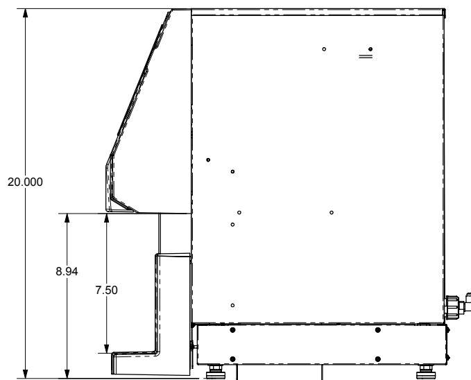
Dimensions of CX with riser
