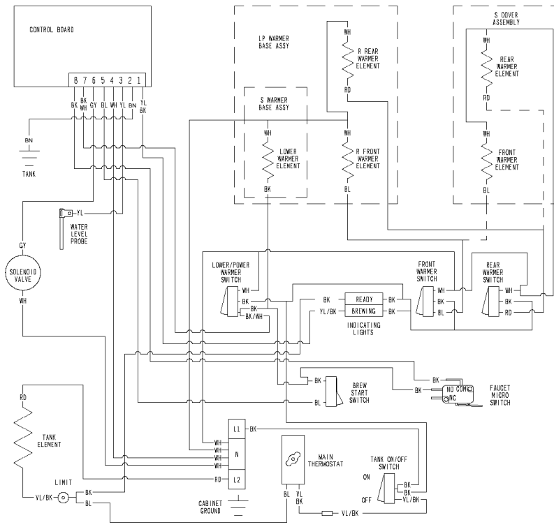
240V WARMER
