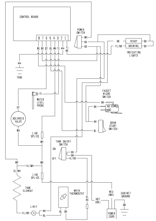
120V DISP.
