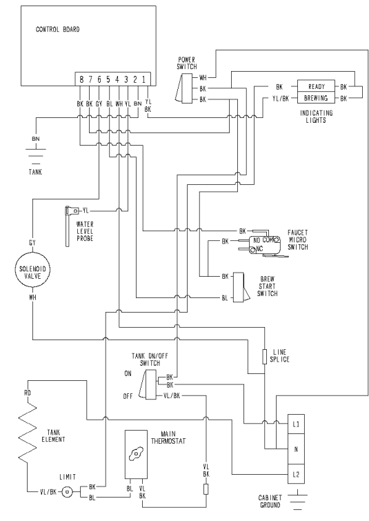
240V DISP.
