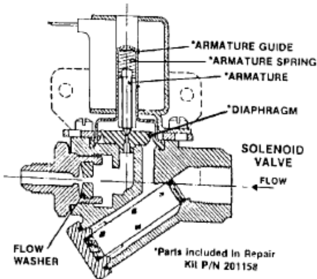
Valve Section View
