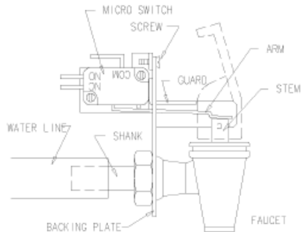
Micro Switch Section View
