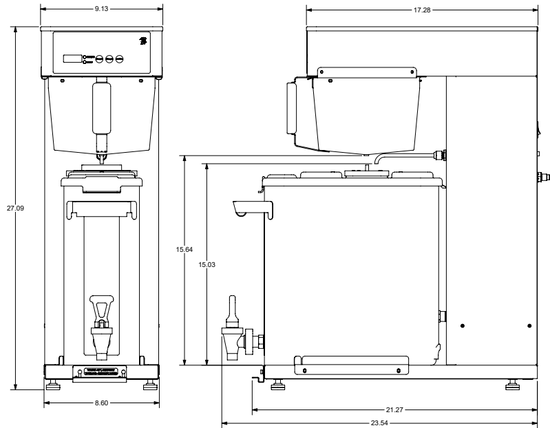
123320 Cold Brew system with (1) 3.5 Gal Dispenser
