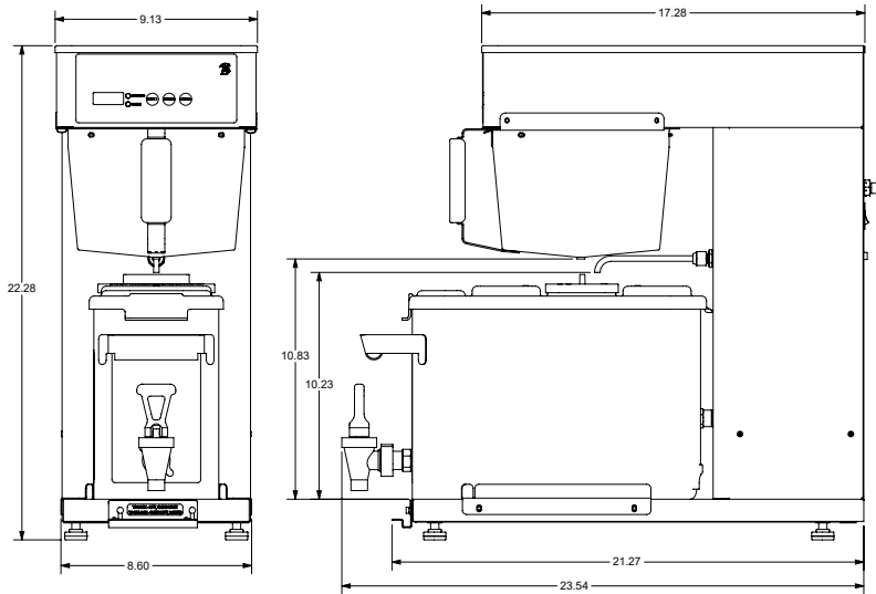
123380 Cold brew System with (1) 2.0 Gal Dispenser
